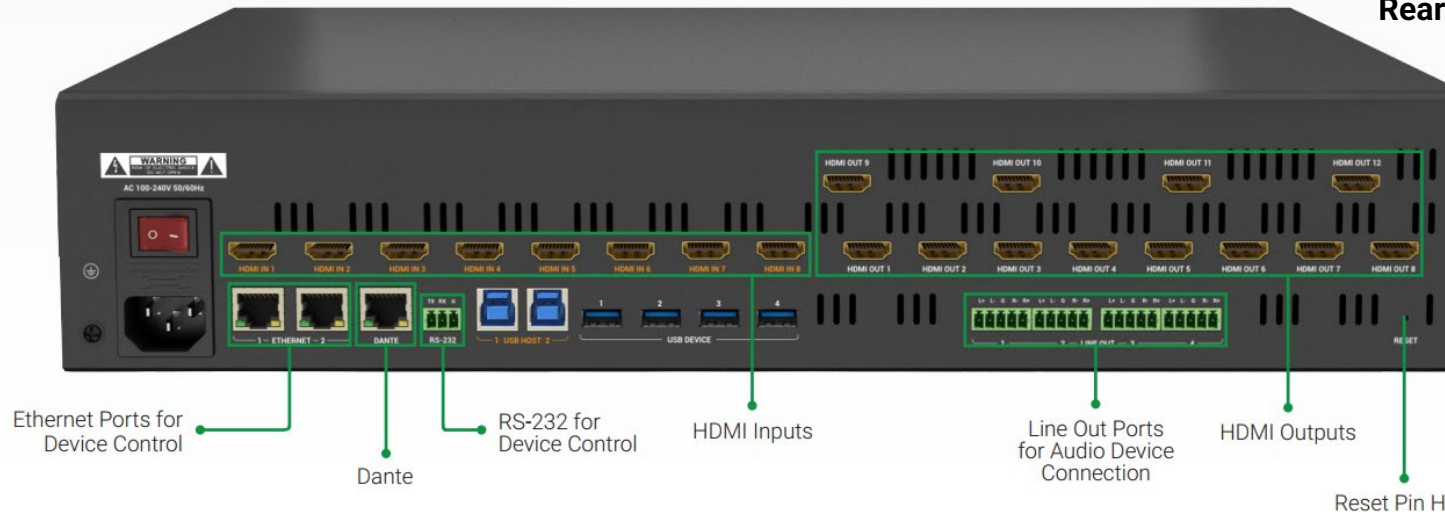
Rear Panel
